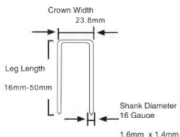
16Ga. Paslode wide crown staple
