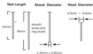
15° Flat wire welded coil nails
